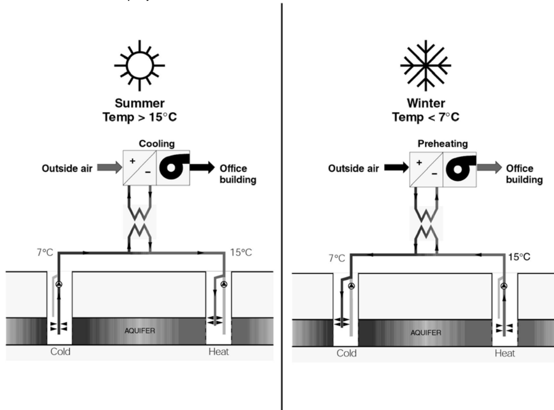
Figure 1. ATEs system integrated with building air-conditioning system.
